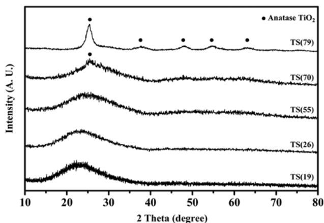
Fig. 1. XRD patterns of TS(X) (X=19, 26, 55, 70, and 79) supports calcined at 550 °C.
