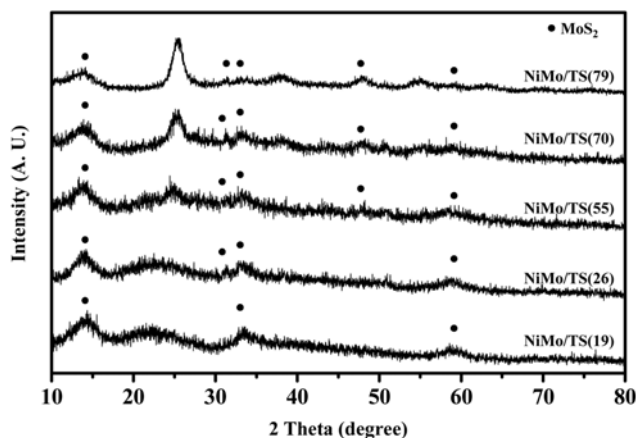
Fig. 2. XRD patterns of NiMo/TS(X) (X=19, 26, 55, 70, and 79) catalysts sulfided at 360 °C.
